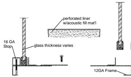
“Split-Frame” Design
