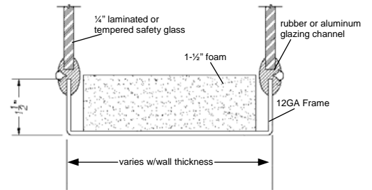
“U” Frame Design
