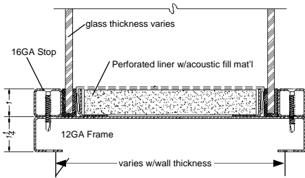
“HM” Frame Design
